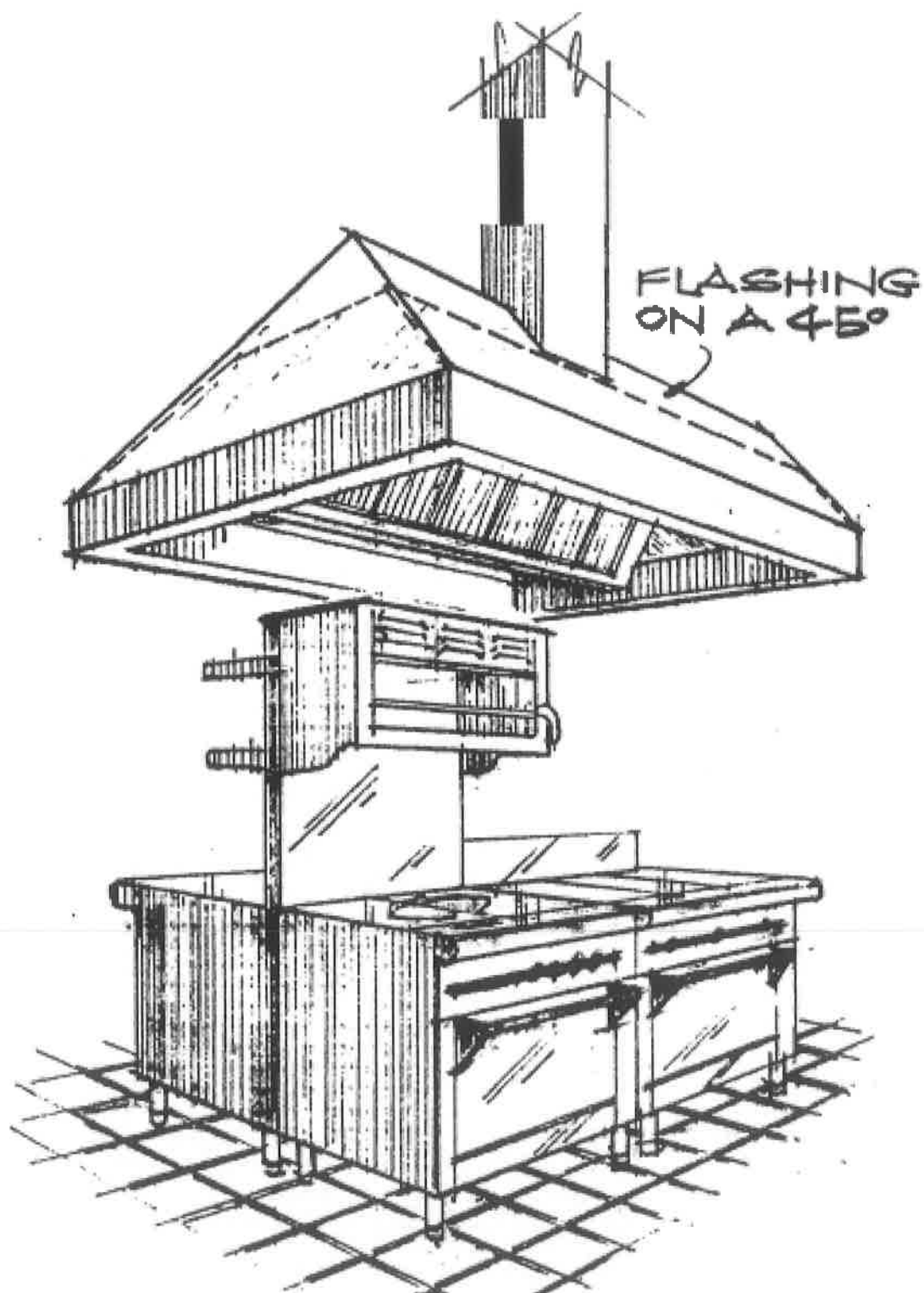
Figure 5. Hood flashing
