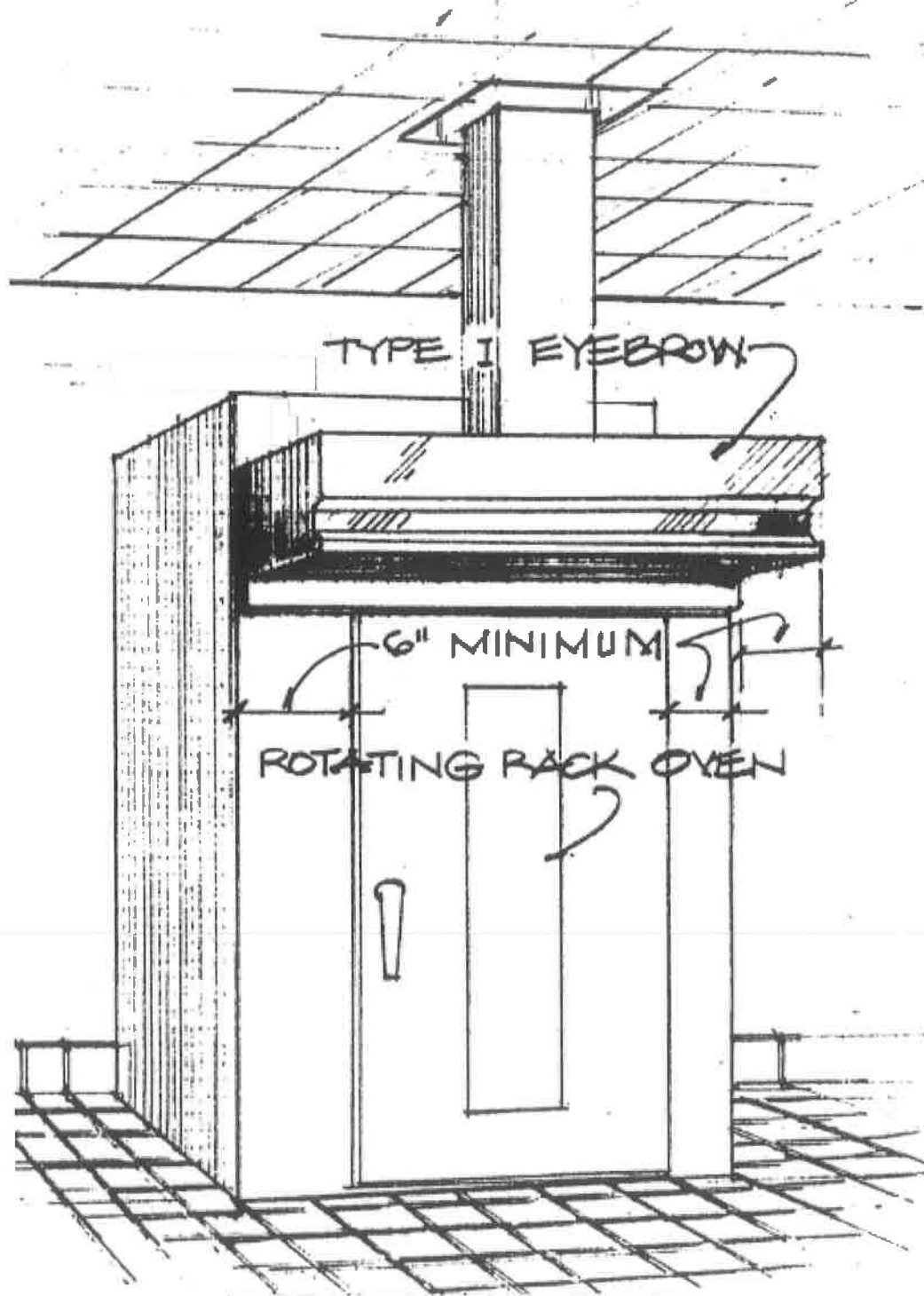
Figure 6. Eyebrow Hood
