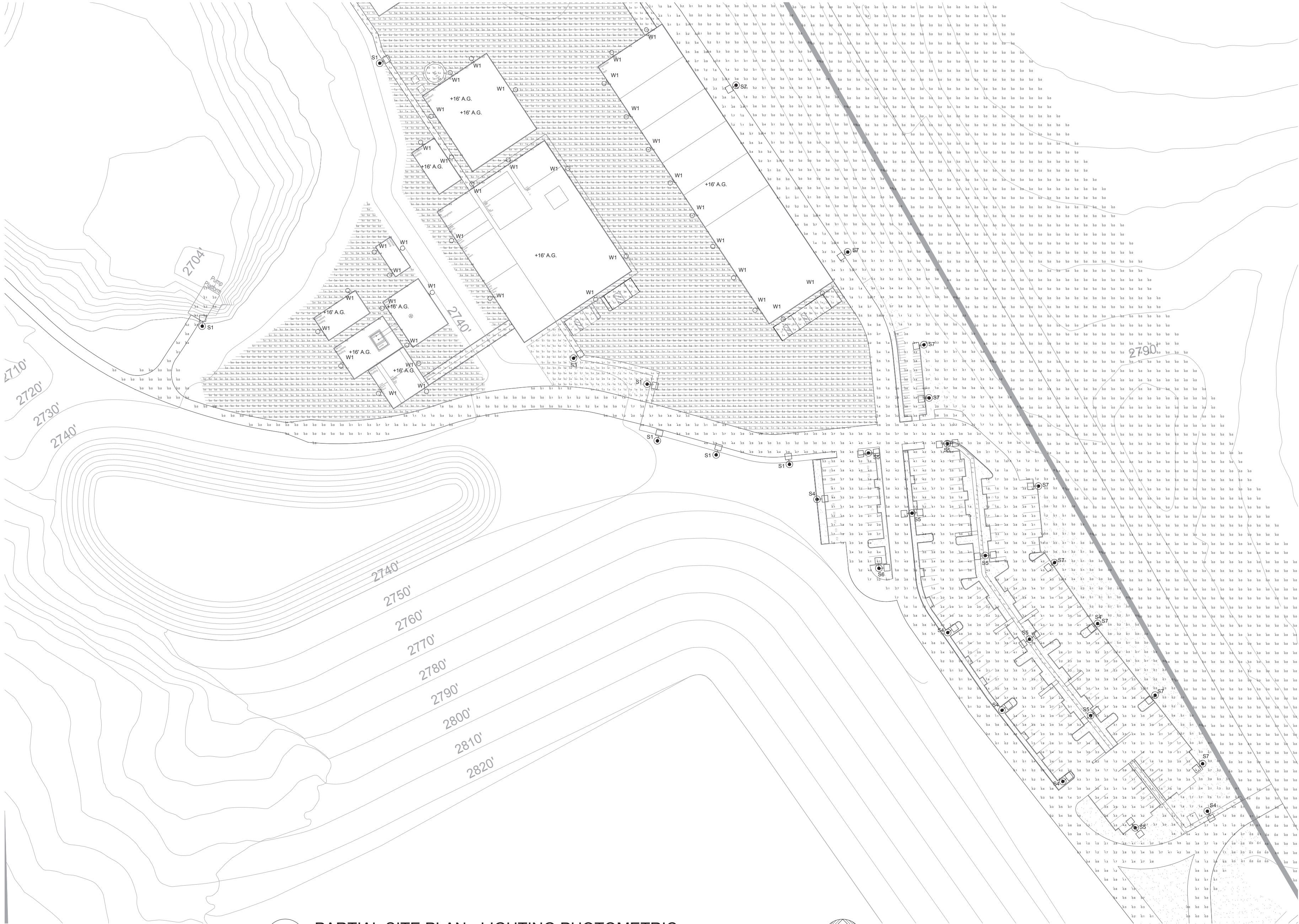
1 E100 PARTIAL SITE PLAN - LIGHTING PHOTOMETRIC SCALE: 1" = 50'-0"
