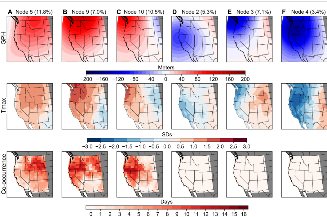
FIG. 3. The six SOM nodes with the largest [(A) to (C)] and smallest [(D) to (F)] PM 2.5 /ozone co-occurrence risk. Top: Geopotential height (GPH) anomalies for each SOM node trained over 1979 to 2020. Middle: Composite standardized anomalies of daily maximum temperatures (T max ) on all days associated with each node during the 2001 to 2020 period. Bottom: Number of times each grid cell experienced local PM 2.5 /ozone co-occurrences during all widespread co-occurrence days associated with that node. The maximum possible number of co-occurrence days in a given grid cell is equivalent to the total number of widespread co-occurrence days associated with that node (node 5, 14 days; node 9, 16 days; node 10, 13 days; Table 1). Values in parentheses on top row indicate the frequency of each SOM node relative to all July to September days during the period of overlap with air pollution data (2001 to 2020).
